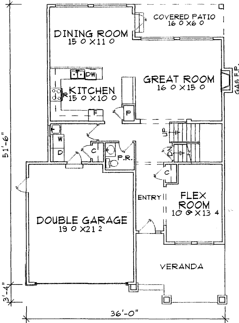
FULL BASEMENT UNDER MAIN FLOOR PLAN FINISHED FLOOR AREA = 1092 sq.ft. GARAGE AREA = 428 sq.ft.
